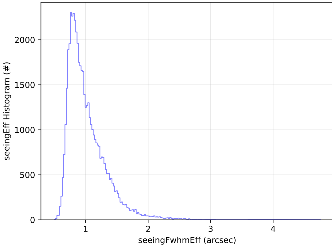
ddf_acor_sf20_lsf40_lsr50_v3.4_10yrs Yr 1 r band: seeingEff Histogram
