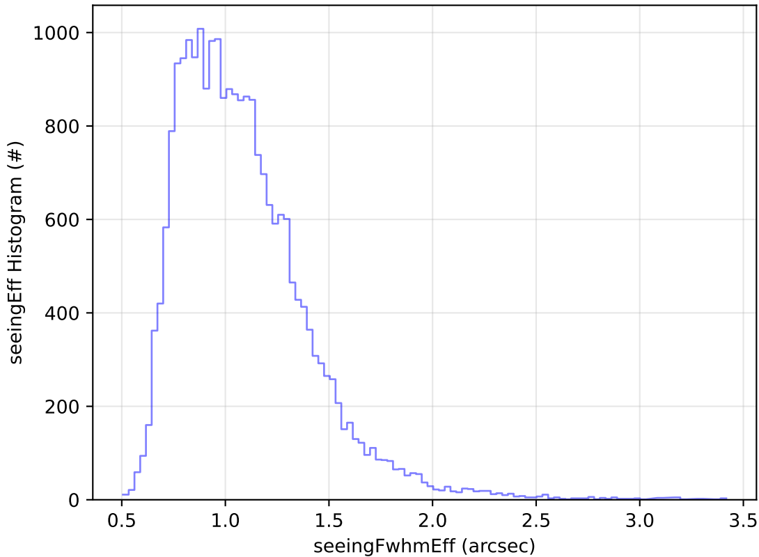
ddf_acor_sf20_lsf40_lsr50_v3.4_10yrs Yr 1 g band: seeingEff Histogram
