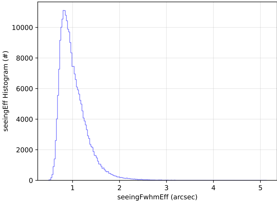
ddf_acor_sf20_Isf40_Isr50_v3.4_10yrs Yr 1 all bands: seeingEff Histogram
