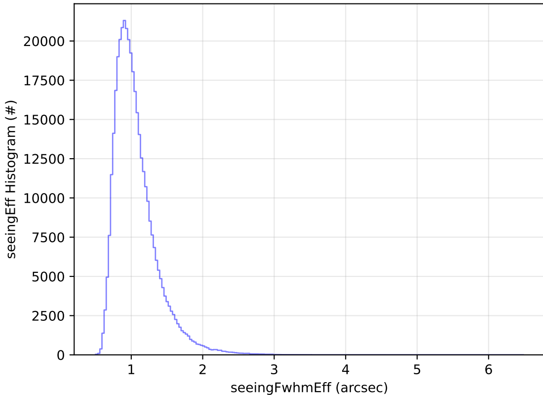
ddf_acor_sf20_lsf40_lsr50_v3.4_10yrs WFD y band: seeingEff Histogram
