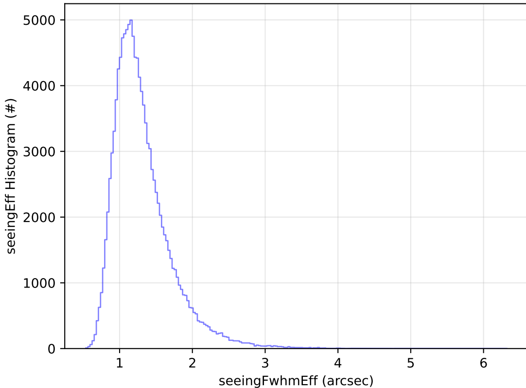
ddf_acor_sf20_lsf40_lsr50_v3.4_10yrs WFD u band: seeingEff Histogram
