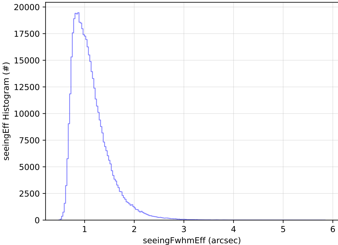
ddf_acor_sf20_lsf40_lsr50_v3.4_10yrs WFD r band: seeingEff Histogram
