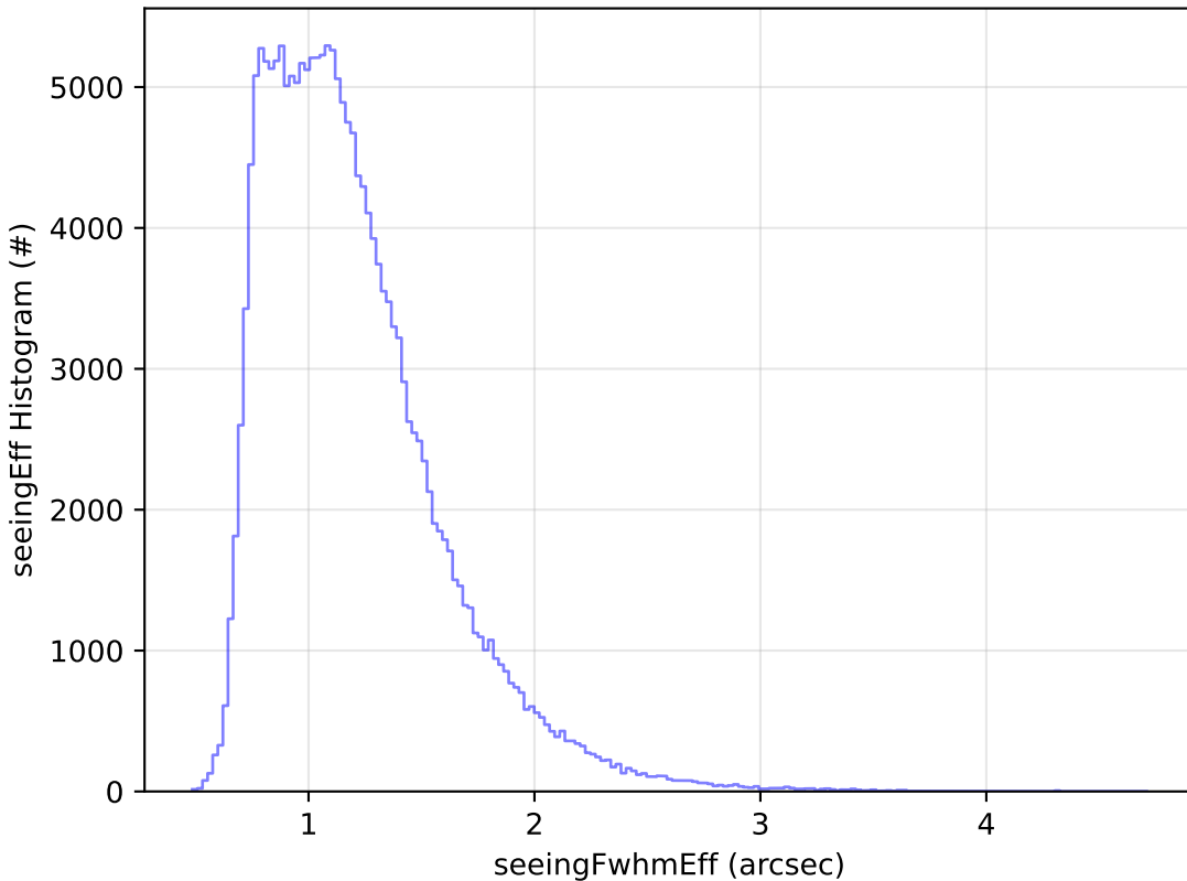
ddf_acor_sf20_lsf40_lsr50_v3.4_10yrs WFD g band: seeingEff Histogram
