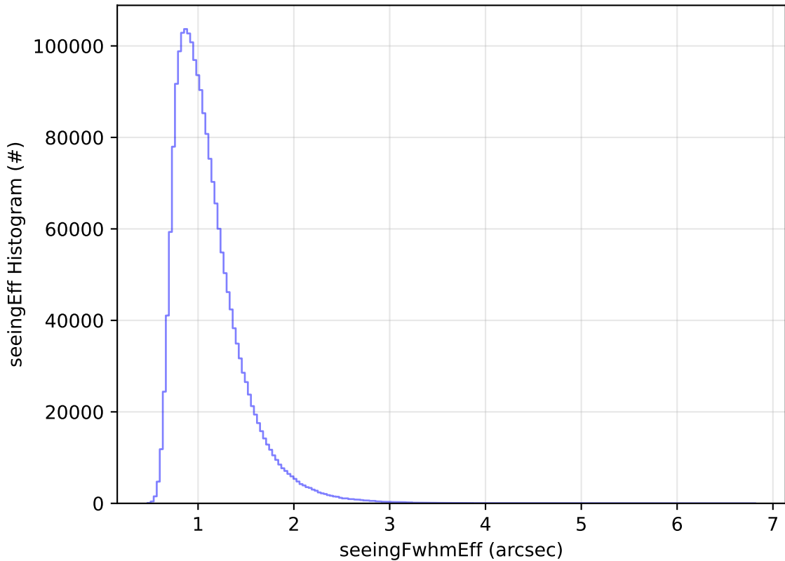
ddf_acor_sf20_lsf40_lsr50_v3.4_10yrs WFD all bands: seeingEff Histogram
