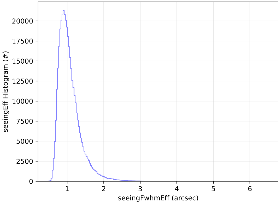
ddf_acor_sf20_lsf40_lsr50_v3.4_10yrs All sky y band: seeingEff Histogram
