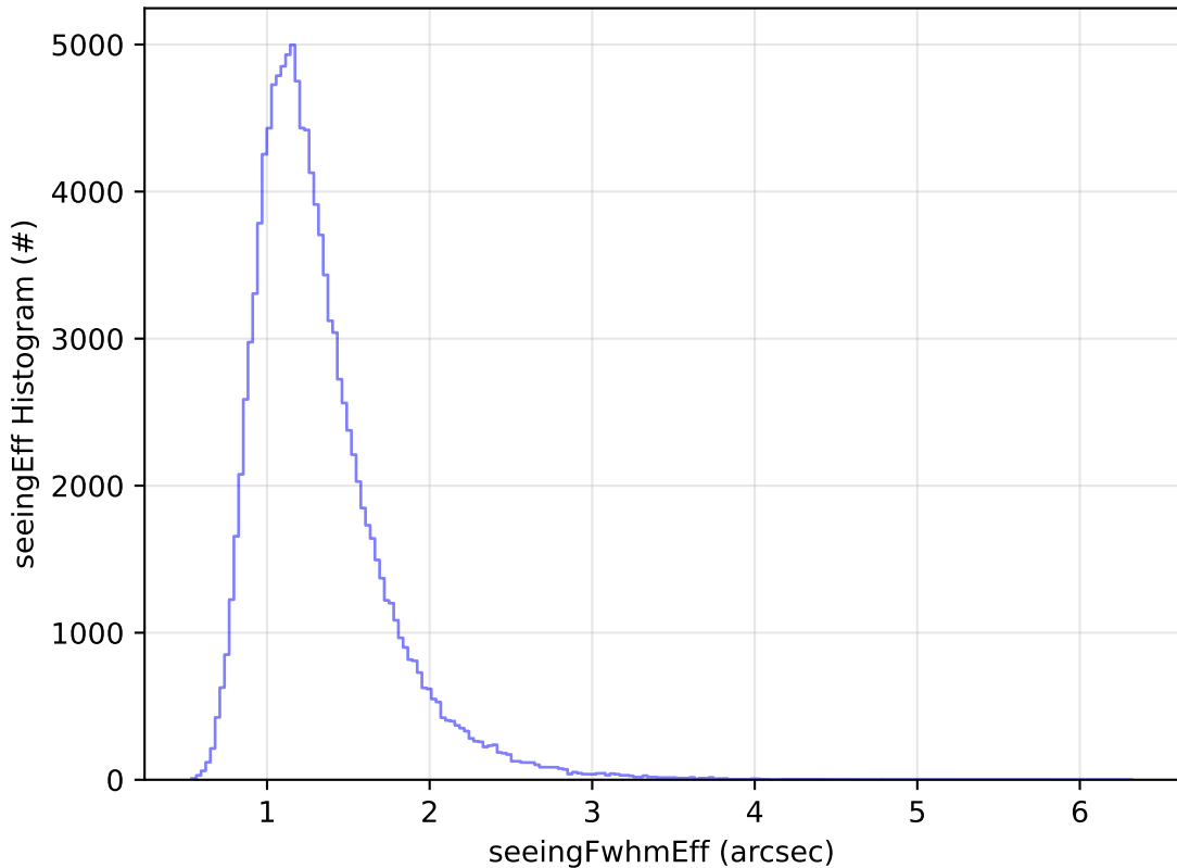
ddf_acor_sf20_ls40_lsr50_v3.4_10yrs All sky u band: seeingEff Histogram
