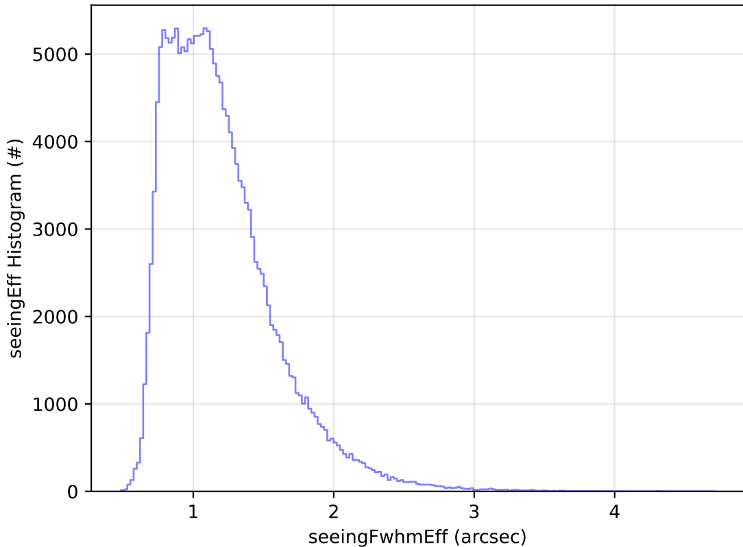
ddf_acor_sf20_ls40_lsr50_v3.4_10yrs All sky g band: seeingEff Histogram
