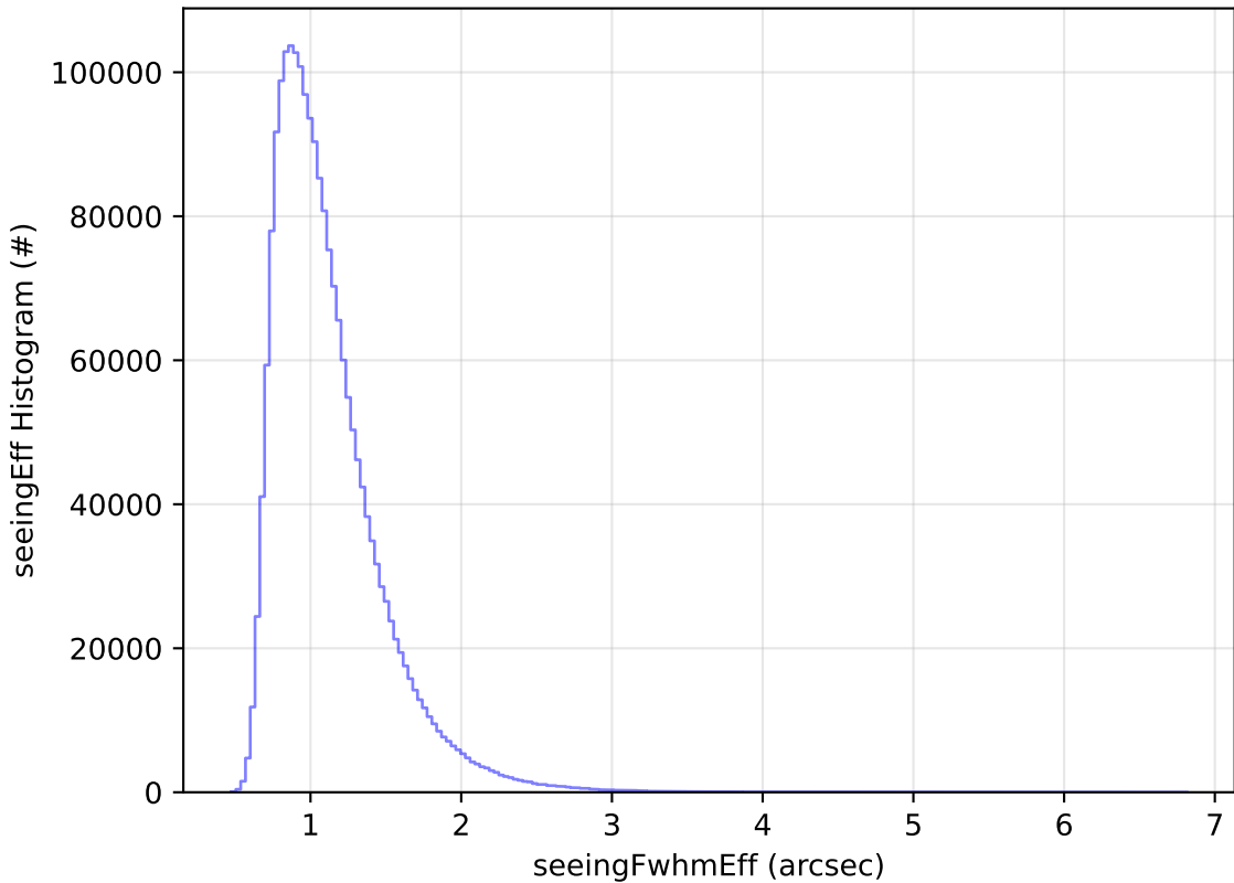
ddf_acor_sf20_lsf40_lsr50_v3.4_10yrs All sky all bands: seeingEff Histogram
