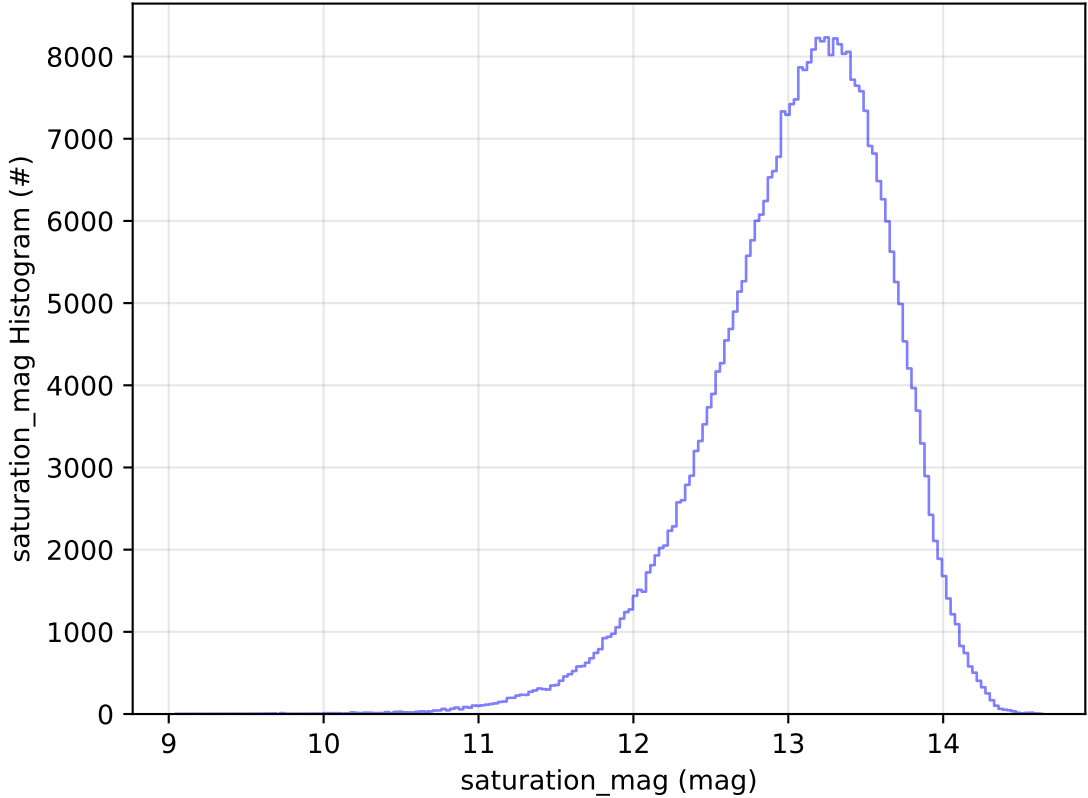
ddf_acor_sf20_lsf40_lsr50_v3.4_10yrs WFD y band: saturation_mag Histogram
