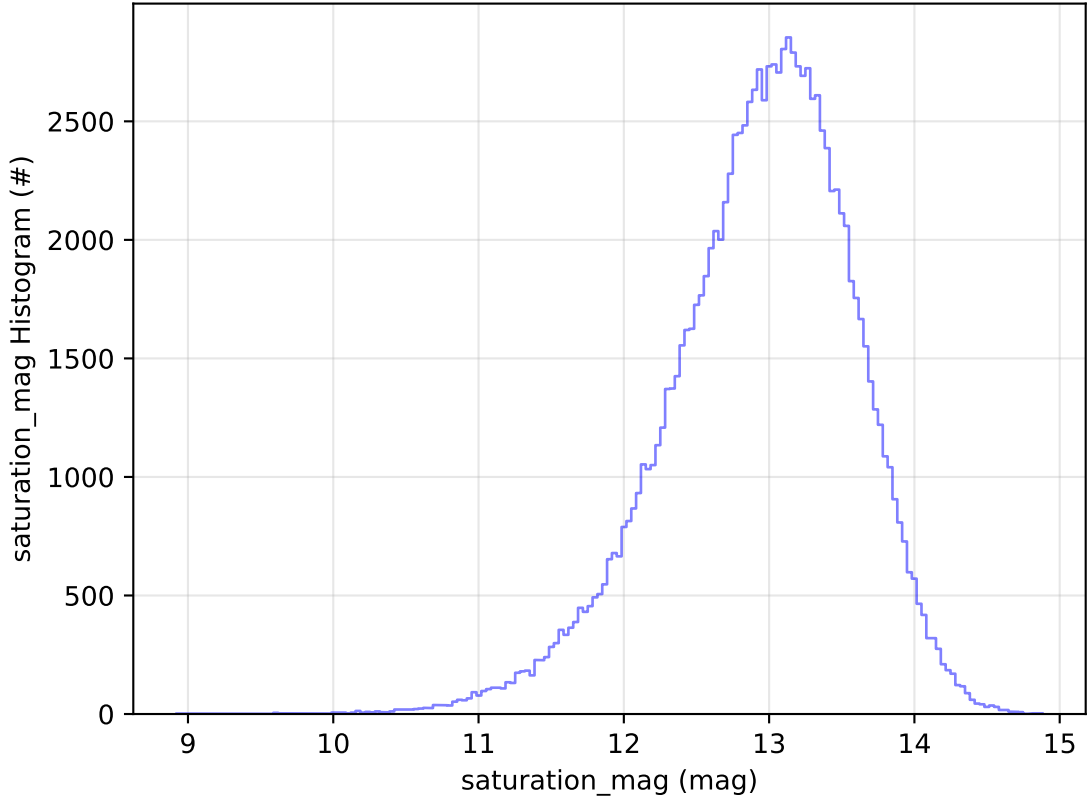
ddf_acor_sf20_lsf40_lsr50_v3.4_10yrs WFD u band: saturation_mag Histogram
