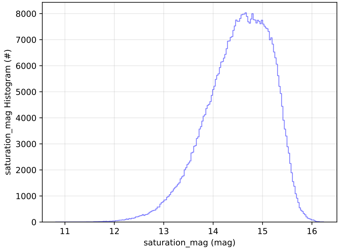
ddf_acor_sf20_lsf40_lsr50_v3.4_10yrs WFD r band: saturation_mag Histogram
