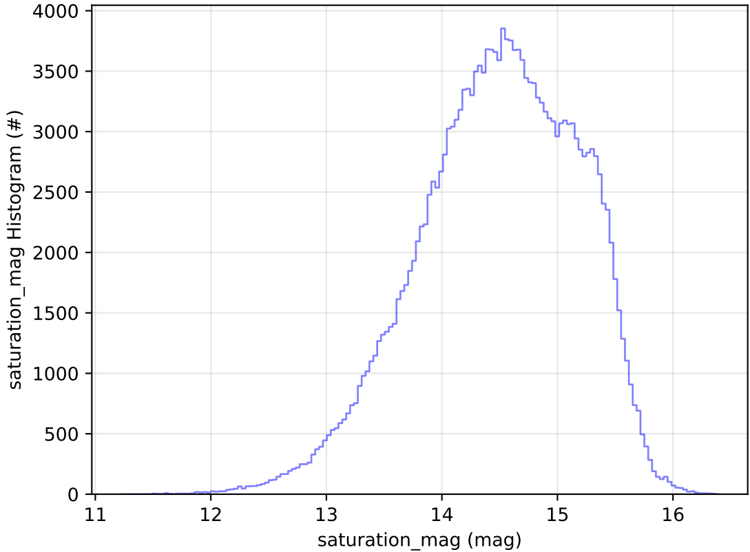
ddf_acor_sf20_lsf40_lsr50_v3.4_10yrs WFD g band: saturation_mag Histogram
