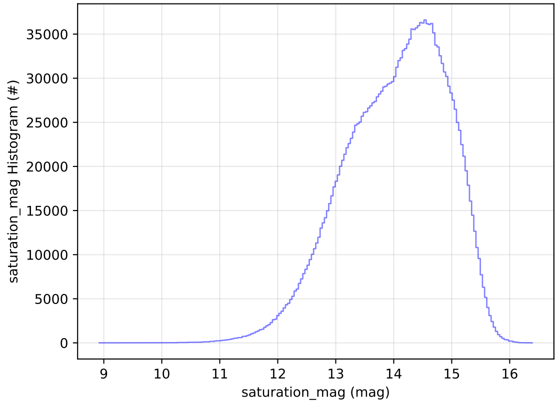
ddf_acor_sf20_lsf40_lsr50_v3.4_10yrs WFD all bands: saturation_mag Histogram
