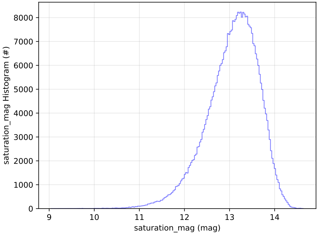
ddf_acor_sf20_lsf40_lsr50_v3.4_10yrs All sky y band: saturation_mag Histogram
