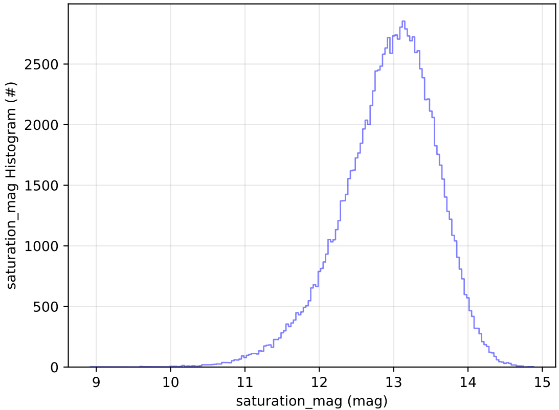
ddf_acor_sf20_lsf40_lsr50_v3.4_10yrs All sky u band: saturation_mag Histogram
