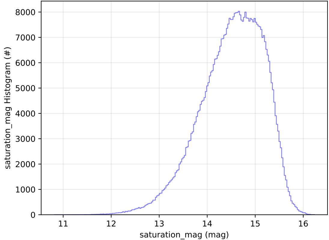
ddf_acor_sf20_lsf40_lsr50_v3.4_10yrs All sky r band: saturation_mag Histogram
