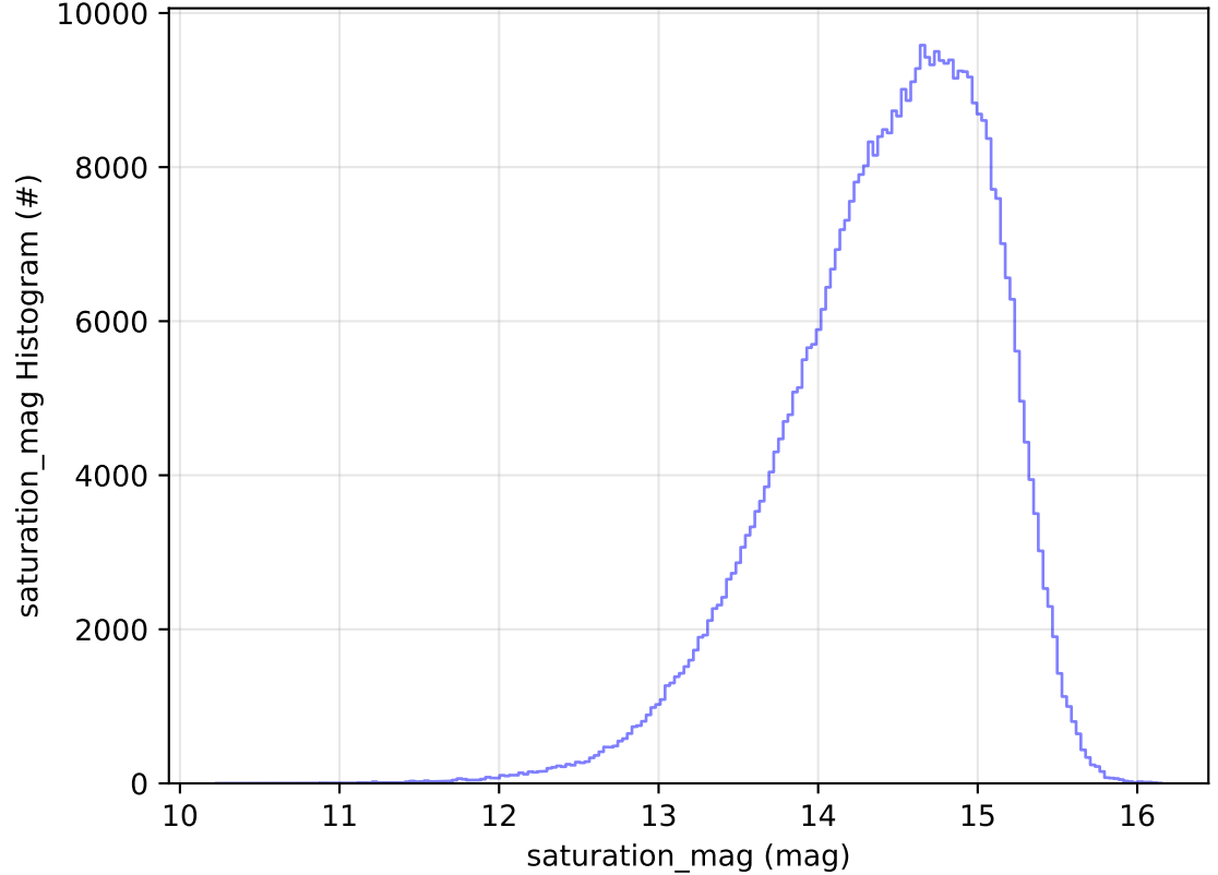
ddf_acor_sf20_lsf40_lsr50_v3.4_10yrs All sky i band: saturation_mag Histogram
