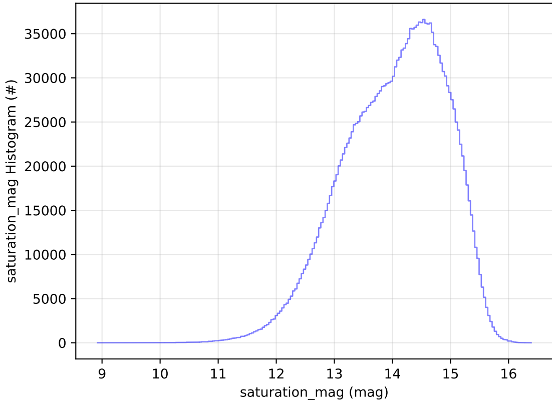
ddf_acor_sf20_lsf40_lsr50_v3.4_10yrs All sky all bands: saturation_mag Histogram
