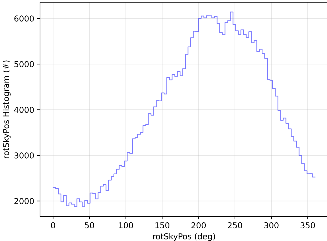
ddf_acor_sf20_lsf40_lsr50_v3.4_10yrs WFD y band: rotSkyPos Histogram
