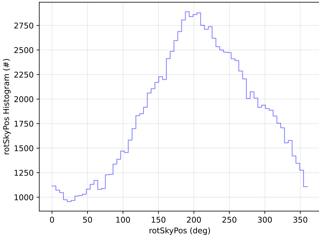
ddf_acor_sf20_lsf40_lsr50_v3.4_10yrs WFD u band: rotSkyPos Histogram
