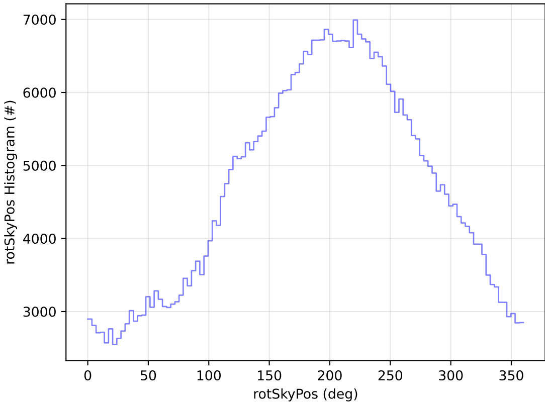
ddf_acor_sf20_lsf40_lsr50_v3.4_10yrs WFD r band: rotSkyPos Histogram
