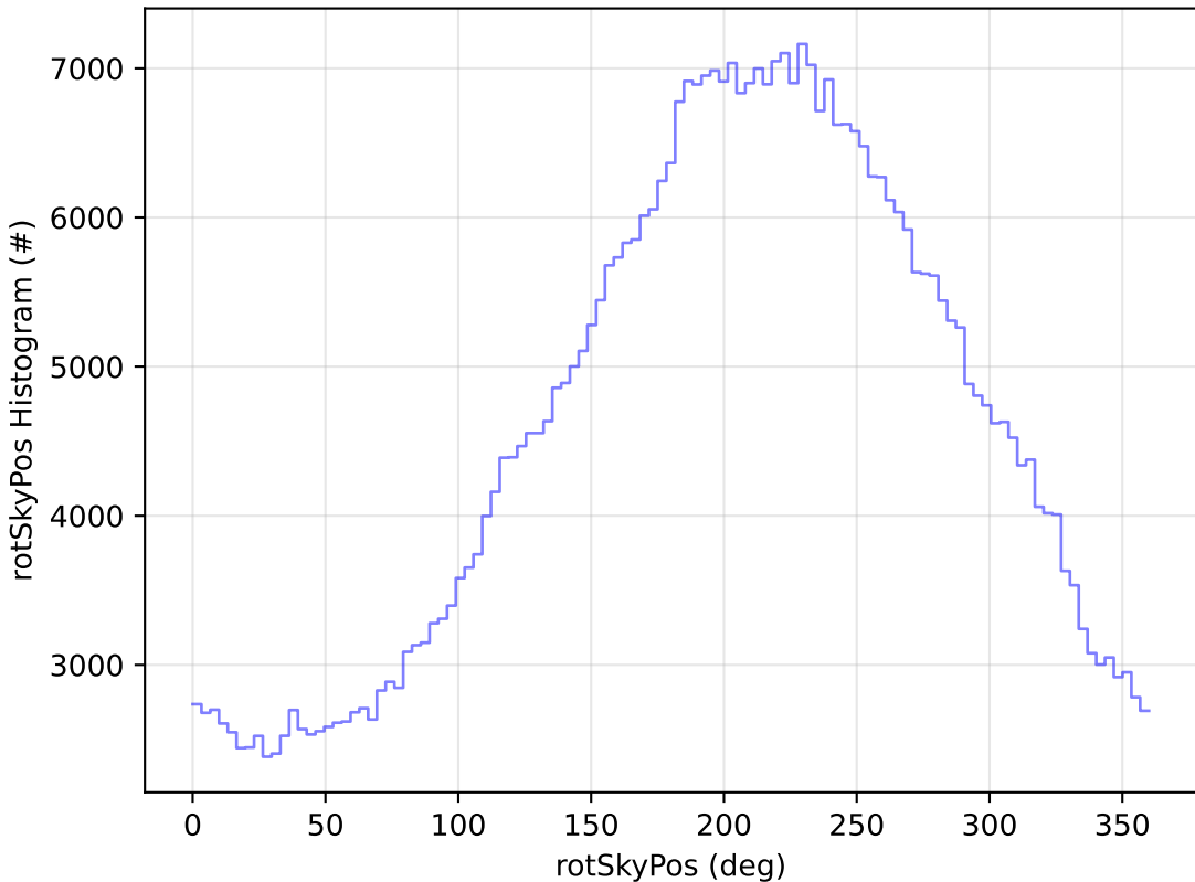
ddf_acor_sf20_lsf40_lsr50_v3.4_10yrs WFD i band: rotSkyPos Histogram
