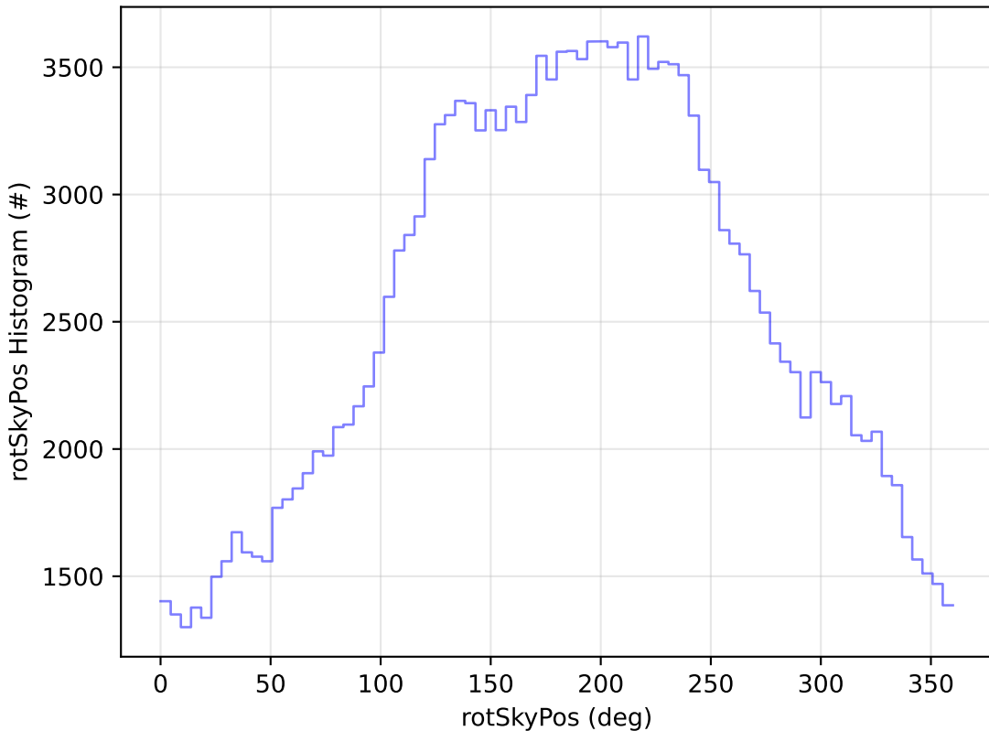
ddf_acor_sf20_lsf40_lsr50_v3.4_10yrs WFD g band: rotSkyPos Histogram
