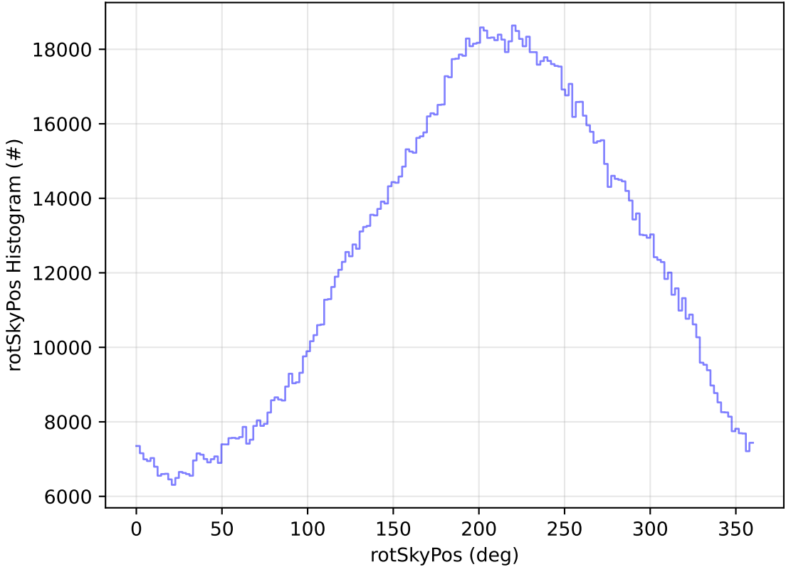
ddf_acor_sf20_lsf40_lsr50_v3.4_10yrs WFD all bands: rotSkyPos Histogram
