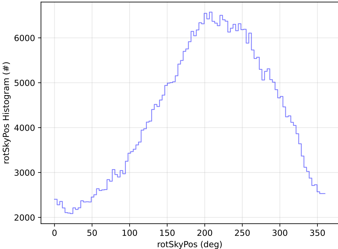
ddf_acor_sf20_lsf40_lsr50_v3.4_10yrs All sky z band: rotSkyPos Histogram
