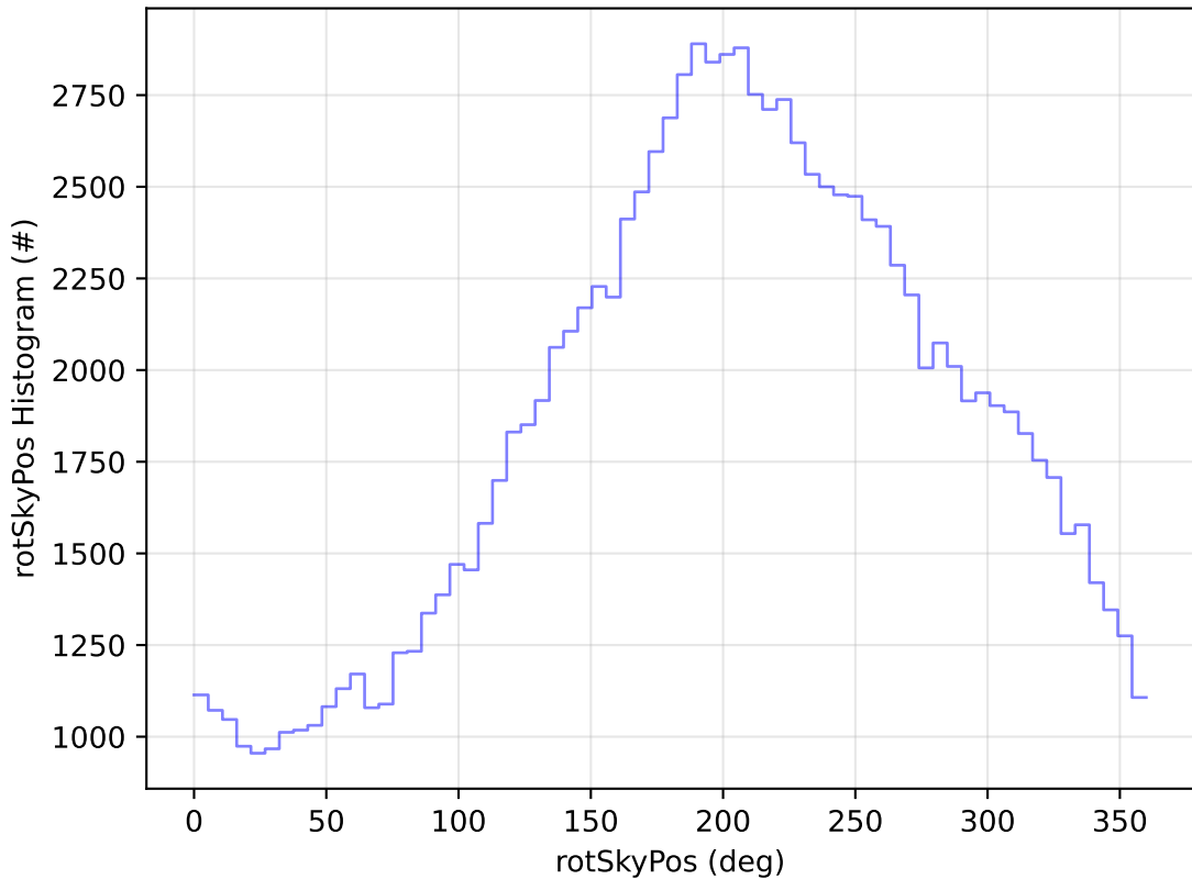
ddf_acor_sf20_lsf40_lsr50_v3.4_10yrs All sky u band: rotSkyPos Histogram
