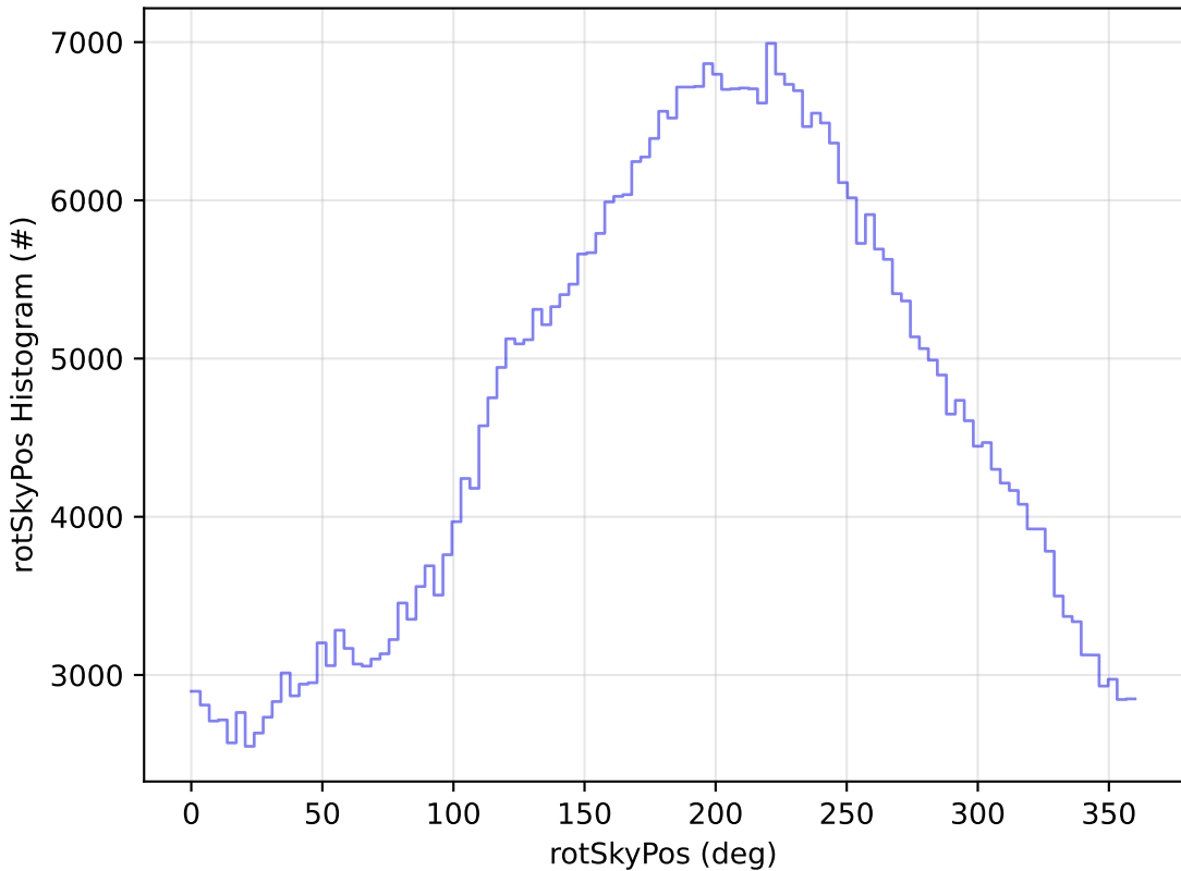
ddf_acor_sf20_ls40_lsr50_v3.4_10yrs All sky r band: rotSkyPos Histogram
