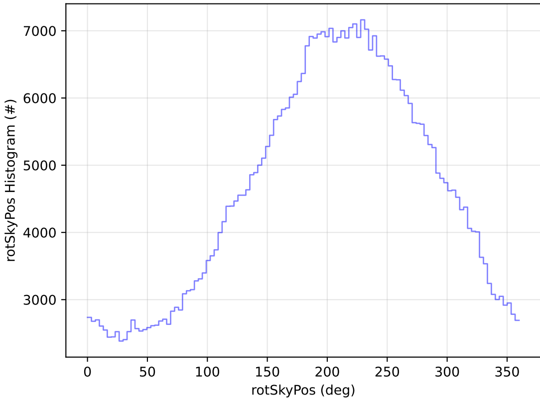
ddf_acor_sf20_lsf40_lsr50_v3.4_10yrs All sky i band: rotSkyPos Histogram
