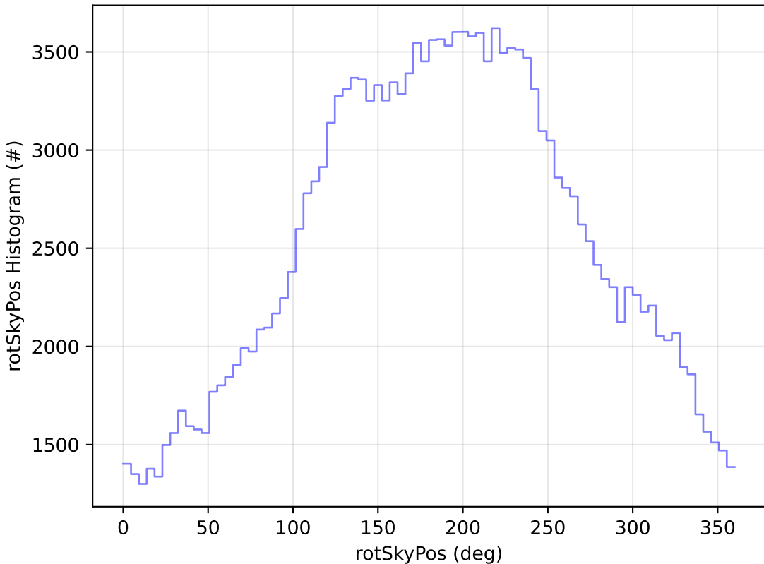
ddf_acor_sf20_lsf40_lsr50_v3.4_10yrs All sky g band: rotSkyPos Histogram
