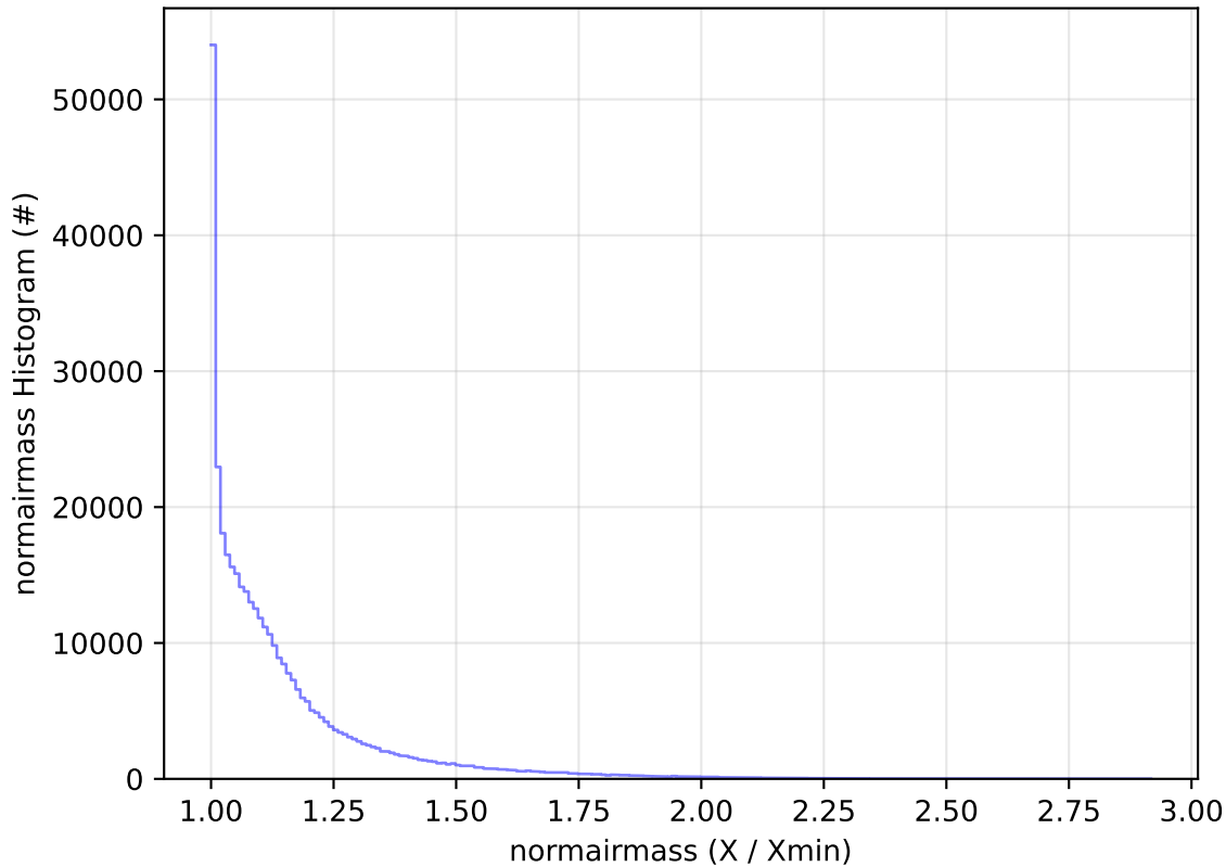
ddf_acor_sf20_lsf40_lsr50_v3.4_10yrs WFD y band: normairmass Histogram
