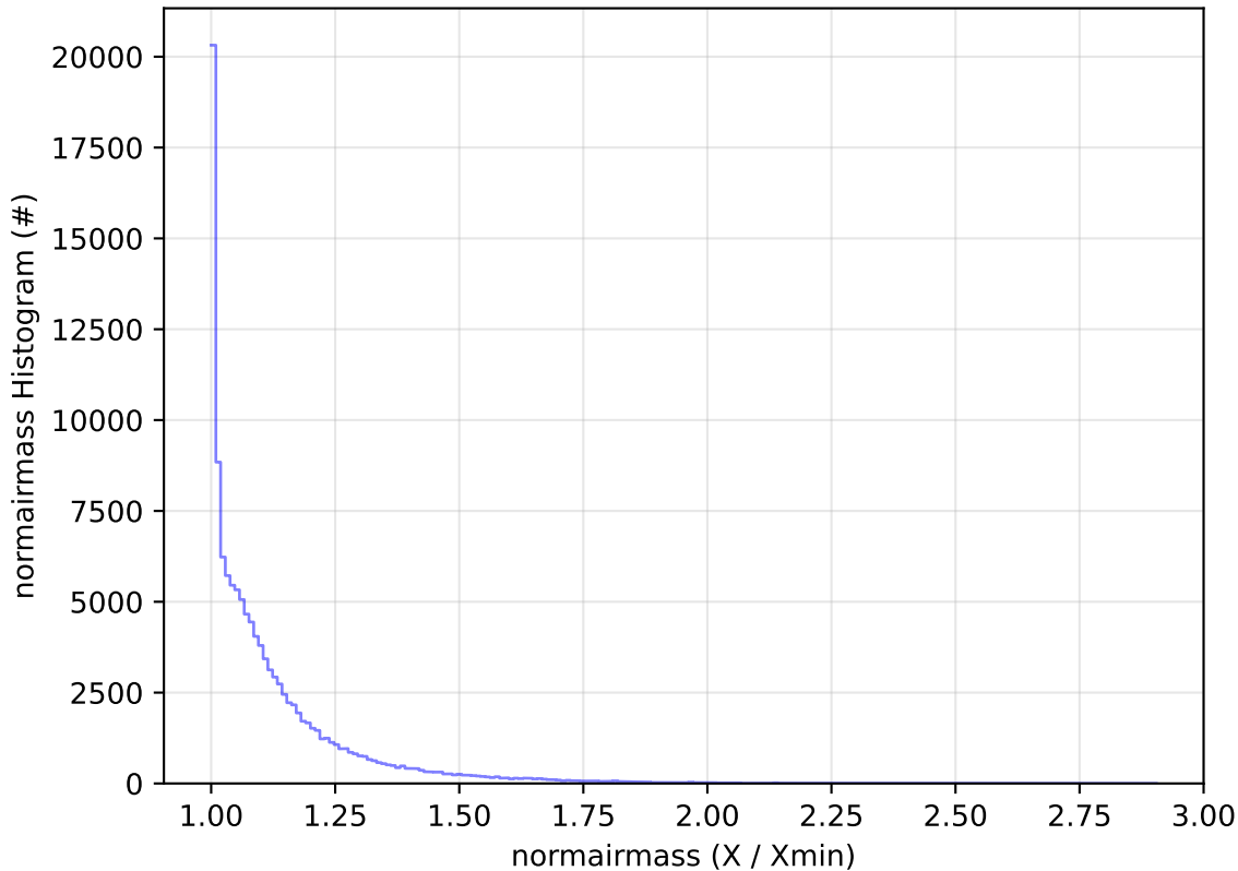
ddf_acor_sf20_lsf40_lsr50_v3.4_10yrs WFD u band: normairmass Histogram
