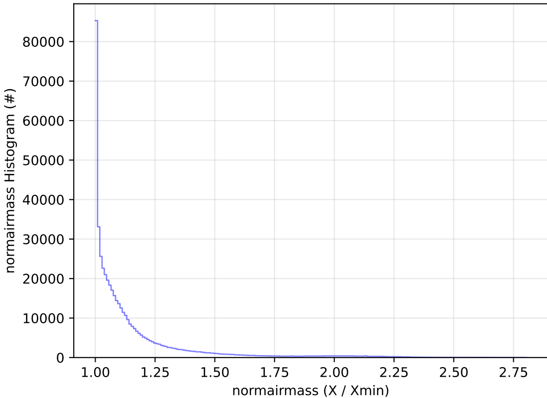
ddf_acor_sf20_lsf40_lsr50_v3.4_10yrs WFD r band: normairmass Histogram
