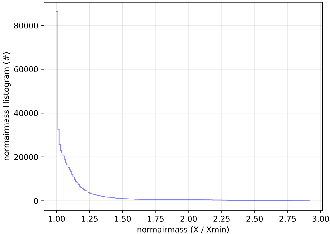
ddf_acor_sf20_lsf40_lsr50_v3.4_10yrs WFD i band: normairmass Histogram
