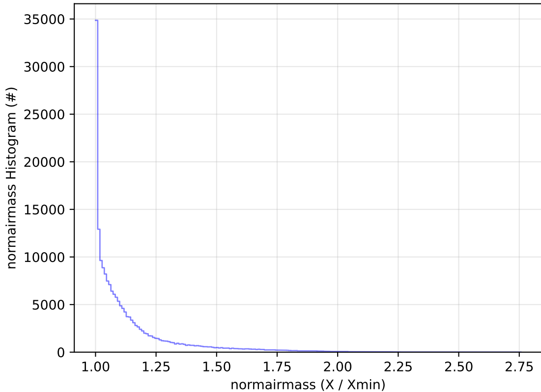
ddf_acor_sf20_lsf40_lsr50_v3.4_10yrs WFD g band: normairmass Histogram
