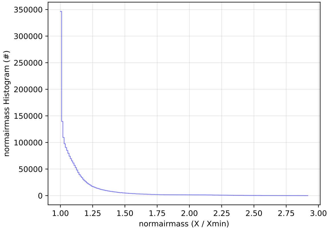
ddf_acor_sf20_lsf40_lsr50_v3.4_10yrs WFD all bands: normairmass Histogram
