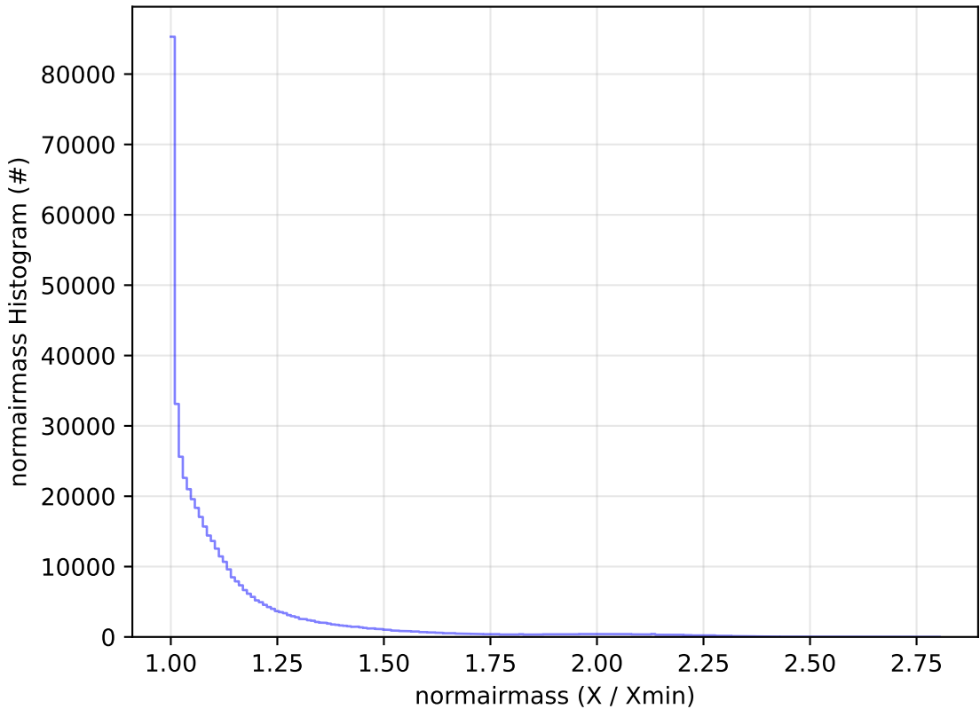
ddf_acor_sf20_lsf40_lsr50_v3.4_10yrs All sky r band: normairmass Histogram
