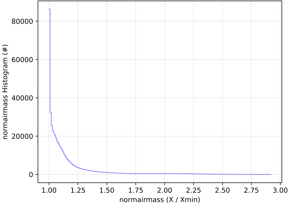
ddf_acor_sf20_lsf40_lsr50_v3.4_10yrs All sky i band: normairmass Histogram
