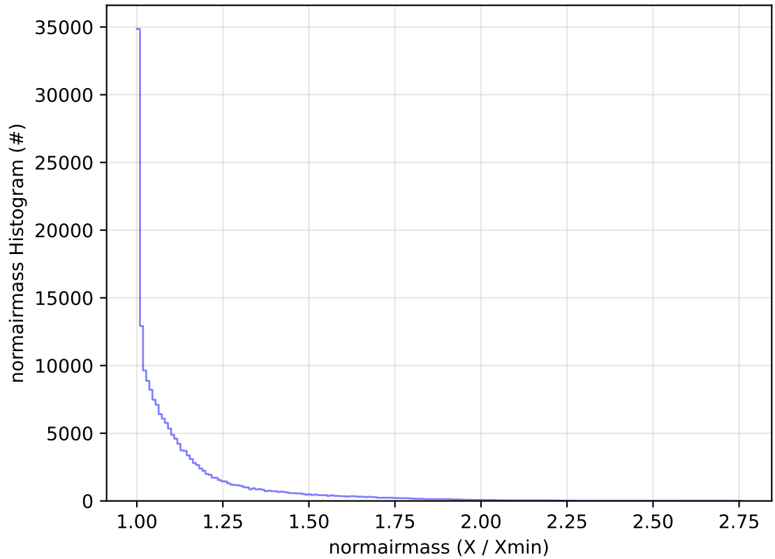
ddf_acor_sf20_lsf40_lsr50_v3.4_10yrs All sky g band: normairmass Histogram
