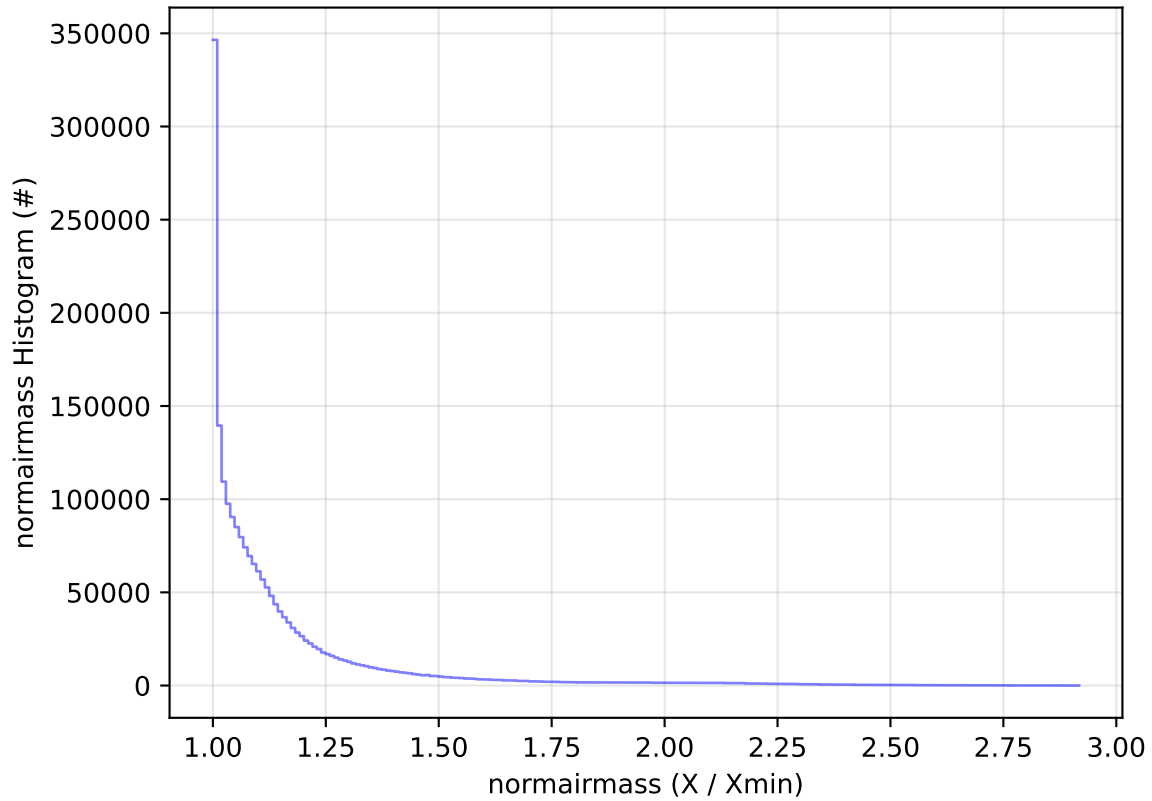
ddf_acor_sf20_lsf40_lsr50_v3.4_10yrs All sky all bands: normairmass Histogram
