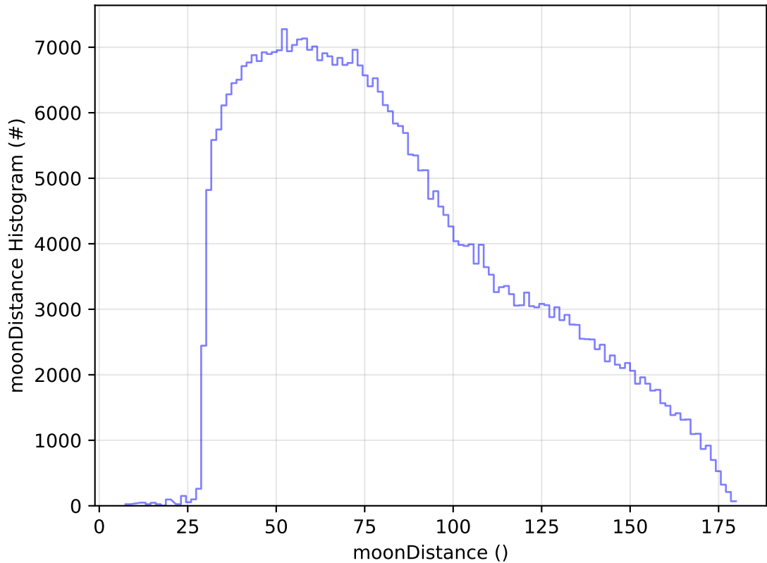
ddf_acor_sf20_lsf40_lsr50_v3.4_10yrs WFD z band: moonDistance Histogram
