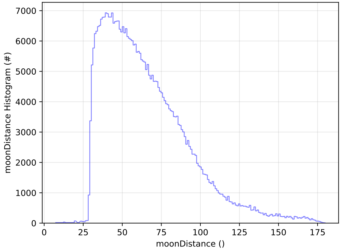
ddf_acor_sf20_Isf40_Isr50_v3.4_10yrs WFD y band: moonDistance Histogram
