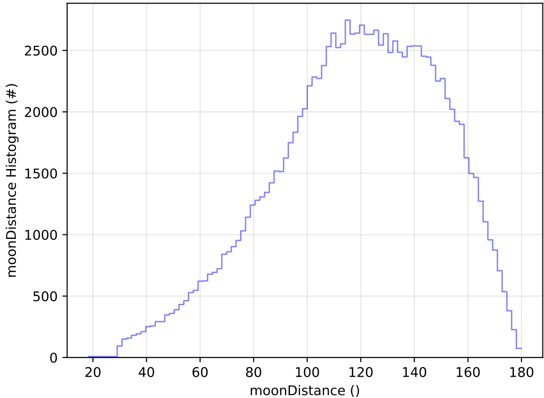
ddf_acor_sf20_lsf40_lsr50_v3.4_10yrs WFD u band: moonDistance Histogram
