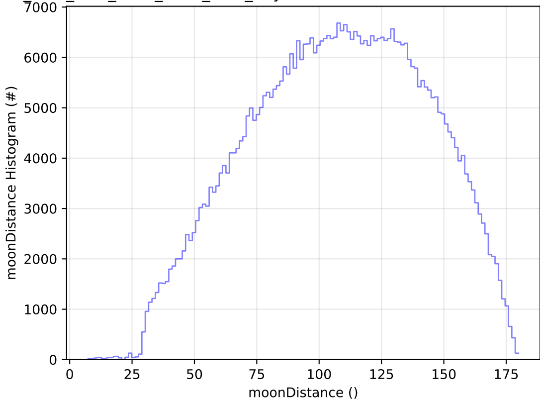
ddf_acor_sf20_lsf40_lsr50_v3.4_10yrs WFD r band: moonDistance Histogram
