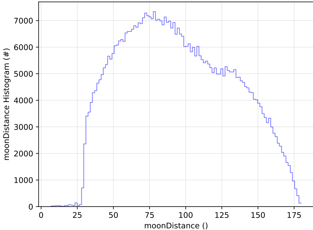
ddf_acor_sf20_lsf40_lsr50_v3.4_10yrs WFD i band: moonDistance Histogram
