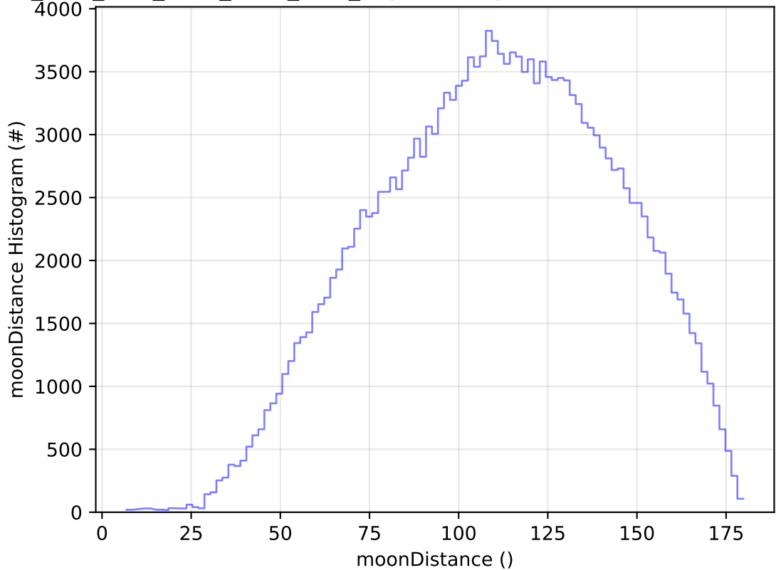
ddf_acor_sf20_lsf40_lsr50_v3.4_10yrs WFD g band: moonDistance Histogram
