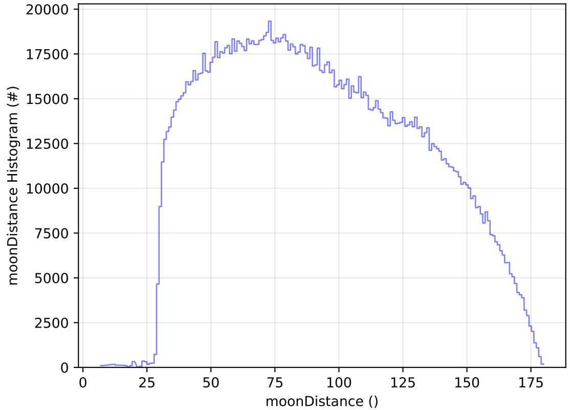
ddf_acor_sf20_lsf40_lsr50_v3.4_10yrs WFD all bands: moonDistance Histogram
